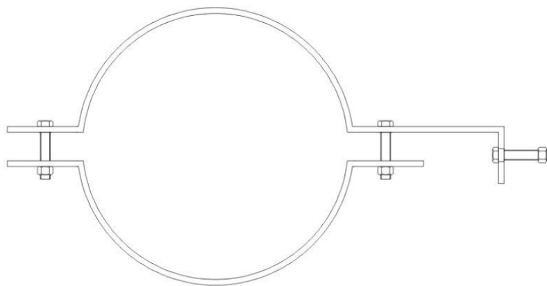
Clevis for Pole 余缆架杆用紧固夹具
